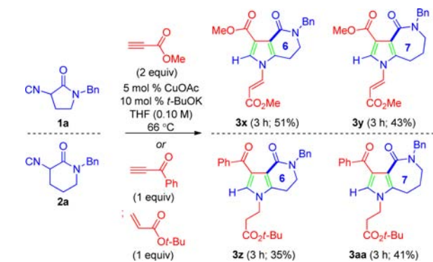
Scheme 3. One-Pot Synthesis of Tetrasubstituted Pyrrololactams
